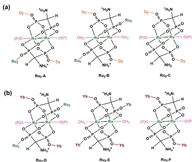
Scheme 3 Coordination modes of \text{Ru}_2(\text{H}_x\text{ampd})_2 dimers in 17 (a) and 18 (b). Reprinted with permission from ref. 24. Copyright 2019, American Chemical Society.
