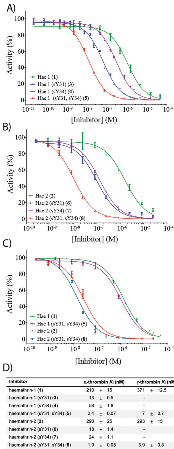
Fig. 2 Dose–response curves for the inhibition of (A) \alpha -thrombin by haemathrin-1 (sulfo)proteins 1 , 3 – 5 ; (B) \alpha -thrombin by haemathrin-2 (sulfo)proteins 2 , 6 – 8 and (C) \gamma -thrombin by unsulfated and doubly sulfated haemathrin-1 and -2 proteins 1 , 2 , 5 and 8 using an amidolytic assay. Error bars represent S.E.M. values; (D) inhibition constants ( K_i , \pm S.E.M.) for haemathrin-1 and -2 (sulfo)proteins. Data were determined by fitting the inhibited steady-state velocities to the Morrison model. 31
