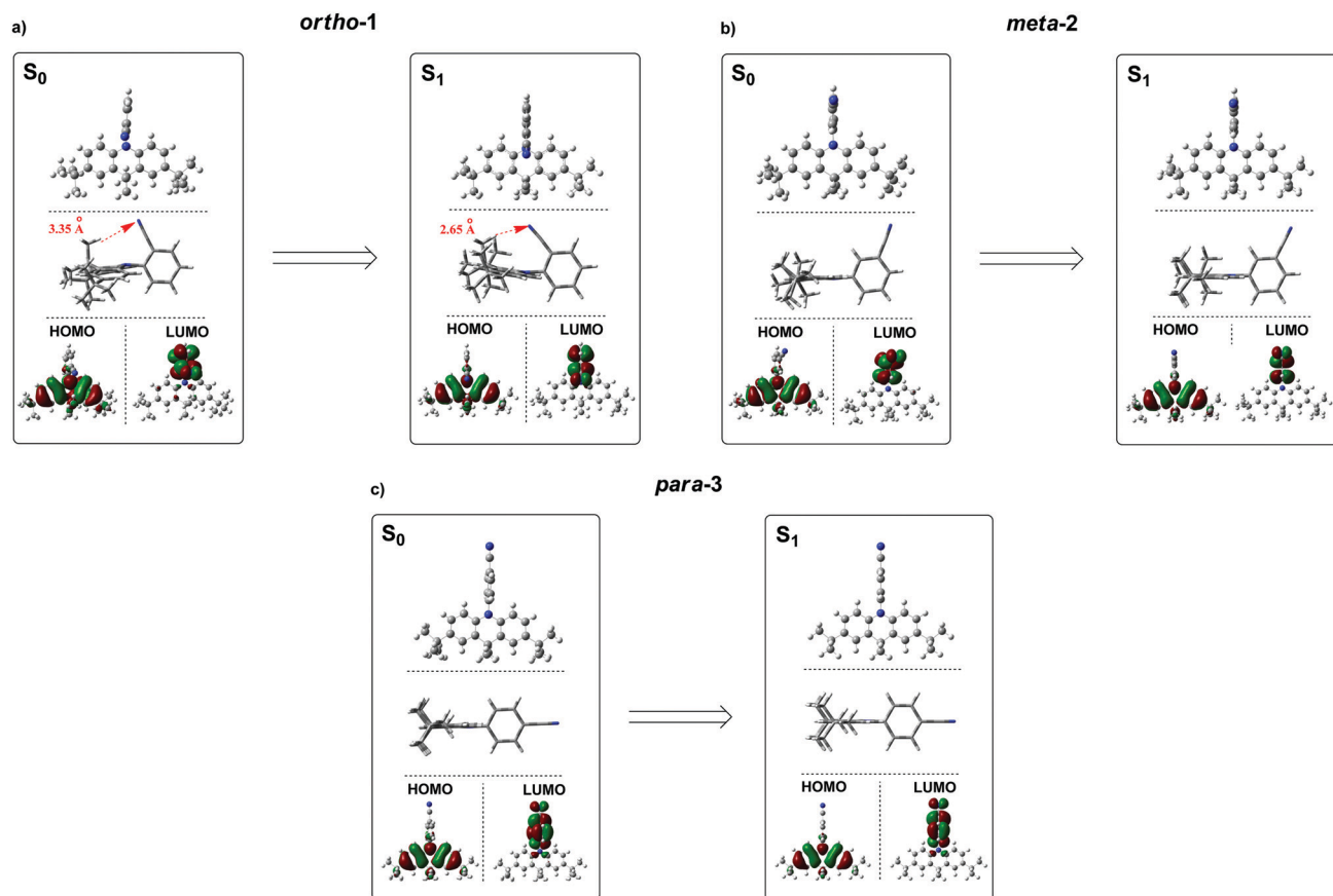
Fig. 4 Ground-state ( S_0 ) and excited-state ( S_1 ) optimised structures of ortho -1, meta -2 and para -3 along with corresponding HOMO/LUMO isosurfaces (rBMK/6-31G(d) for S_0 and TDA-DFT BMK/6-31G(d) the S_1 ).
