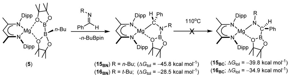
Scheme 4 Synthesis of compounds 15_{\text{BN}} and 16_{\text{BN}} with their DFT-computed energies relative to complex 5 and those of the experimentally unobserved magnesium amide isomers, 15_{\text{BC}} and 16_{\text{BC}} .
