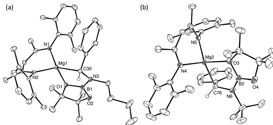
Fig. 2 ORTEP representations (25% probability ellipsoids) of (a) compound 15_{\text{BN}} and (b) the Mg2-containing molecule of compound 16_{\text{BN}} . Hydrogen atoms except for those attached to C30 ( 15_{\text{BN}} ) and C76 ( 16_{\text{BN}} ), iso-propyl methyl groups and the Mg1-containing molecule of compound 16_{\text{BN}} have been removed for clarity. Selected bond lengths (Å) and angles (°): ( 15_{\text{BN}} ) Mg1–N1 2.0460(11), Mg1–N2 2.0301(11), Mg1–C30 2.1549(13), Mg1–O1 2.1250(9), N3–B1 1.3904(18), N3–C30 1.4754(16), N2–Mg1–N1 96.36(4), N2–Mg1–C30 123.40(5), N1–Mg1–O1 107.37(4), N1–Mg1–C30 129.17(5), N2–Mg1–O1 116.00(4), N2–Mg1–N1 96.36(4), N3–B1–O1 121.82(12); ( 16_{\text{BN}} ) Mg2–O3 2.1061(13), Mg2–N4 2.0660(15), Mg2–N5 2.0556(15), Mg2–C76 2.1668(18), O3–B2 1.426(3), N6–C76 1.474(2), N6–B2 1.388(3), O3–Mg2–C76 82.44(6), N4–Mg2–O3 118.29(6), N4–Mg2–C76 114.77(7), N6–C76–Mg2 108.67(11), N6–B2–O3 122.30(17).
