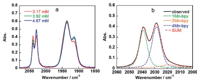
Fig. 5 IR spectra of \text{fac-[Mn(bpy)(CO)}_3(\text{MeCN})]^+ in DMF containing 1.3 M TEOA and different concentrations of \text{CO}_2 (a) and the curve-fitting result for the observed spectra at 3.17 mM \text{CO}_2 (b).
