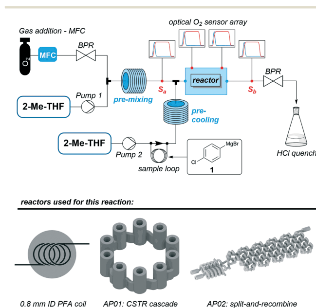
Fig. 11 General scheme of the reaction set-up to carry out the aerobic oxidation of 1 in three different reactors including the positioning of the optical oxygen sensors.
