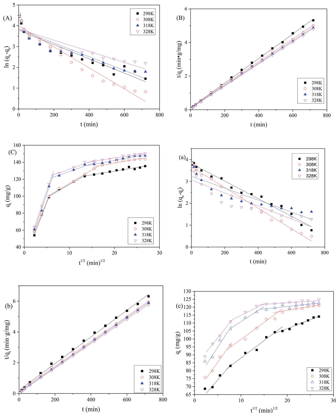
Fig. 9 (A) Pseudo-first-order kinetic model; (B) pseudo-second-order kinetic model; and (C) intraparticle diffusion model for the adsorption of MB on MAC at the initial concentration of 250 mg L; and (a) pseudo-first-order kinetic model; (b) pseudo-second-order kinetic model; and (c) intraparticle diffusion model for the adsorption of MB on MAC at the initial concentration of 150 mg L -1 .
