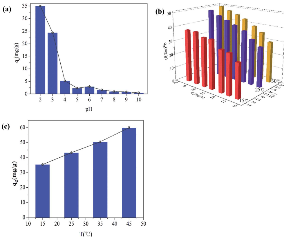
Fig. 9 Effect of pH on Cr(vi) removal ( C_0 = 16.63 \text{ mg L}^{-1} ; dose of \text{Fe}_2\text{O}_3/\text{rGO} = 0.4 \text{ g L}^{-1} ; T = 25 \pm 1^\circ\text{C} ; t = 36 \text{ h} ; 140 rpm) (a); effect of the initial Cr(vi) concentration (b); effect of the temperatures (c) (dose of \text{Fe}_2\text{O}_3/\text{rGO} = 0.4 \text{ g L}^{-1} ; pH = 2.2; t = 36 \text{ h} ; 140 rpm).
