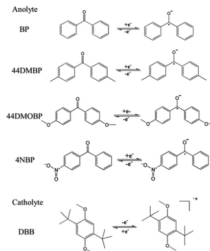
Scheme 1 Redox reactions of the anolytes and catholyte.
