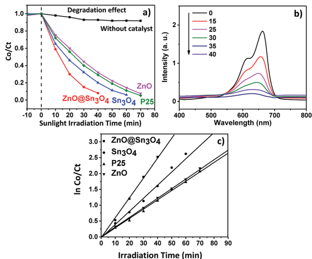
Fig. 9 (a) Plot of change in absorbance vs. irradiation time in the presence of ZnO, Sn 3 O 4 , P25 and ZnO@Sn 3 O 4 ; (b) spectral changes of degradation of MB dye in the presence of ZnO@Sn 3 O 4 ; (c) pseudo-first-order kinetic plots of \ln(C_0/C_t) vs. irradiation time for the degradation of methylene blue (MB) using ZnO, Sn 3 O 4 , P25 and ZnO@Sn 3 O 4 .
