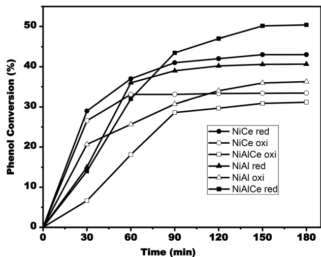
Fig. 15 Evolution of phenol conversion during single run catalytic tests for NiAlCe oxi ( \square ), NiAlCe red ( \blacksquare ), NiAl oxi ( \triangle ), NiAl red ( \blacktriangle ), NiCe oxi ( \circ ), NiCe red ( \bullet ).
