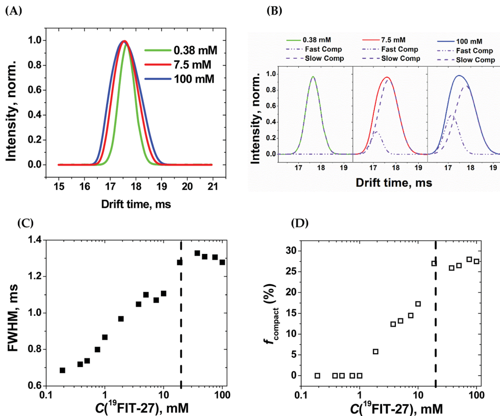
Fig. 5 Ion-mobility mass-spectrometry (IM-MS) characterization of 19 FIT-27 at different concentrations. (A) Concentration-dependent changes in spectral peak width for [ 19 FIT-27]Na + ; (B) single- and two-Gaussian deconvolution of the ion peaks shown in (A). The slow component has drift time of 17.9 ms; the fast component, 17.2 ms; (C) dependence of the full width at half-maximum (FWHM) of the ion peaks shown in (A) vs. C(^{19}\text{FIT-27}) ; and (D) fraction of faster drifting compact form, f_{\text{compact}} , of [ 19 FIT-27]Na + vs. C(^{19}\text{FIT-27}) . The vertical dashed line in (C) and (D) highlights the transition point of ~20 mM in the gas phase.
