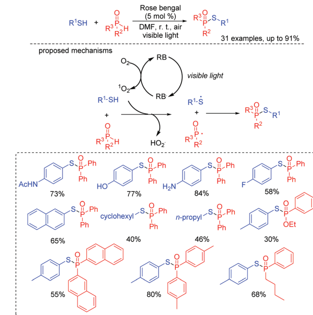
Scheme 24 Construction of S–P(O) bonds.
