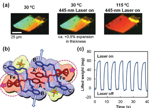
Fig. 15 (a) Optical micrographs of a single crystal of 1 under polarized light. (b) Molecular structure of 1 and its photoinduced motion by 445 nm laser irradiation. (c) Time dependence of lifting weight of the crystal induced by 445 nm focused laser irradiation at 30 °C.
