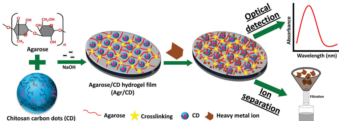
Fig. 6 Fabrication of an agarose/carbon-dot/hydrogel film optical sensor for heavy metal ion detection. 17
