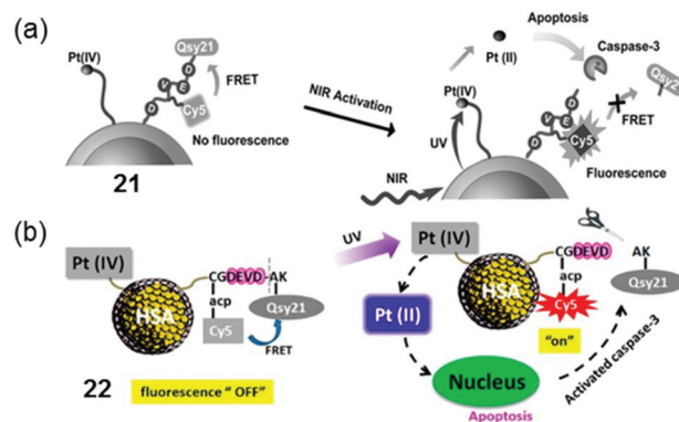
Fig. 13 Photoactivation of conjugates 21 and 22 based on (a) UCNP 117 and (b) HSA, 118 respectively. Adapted from ref. 117 and 118.
