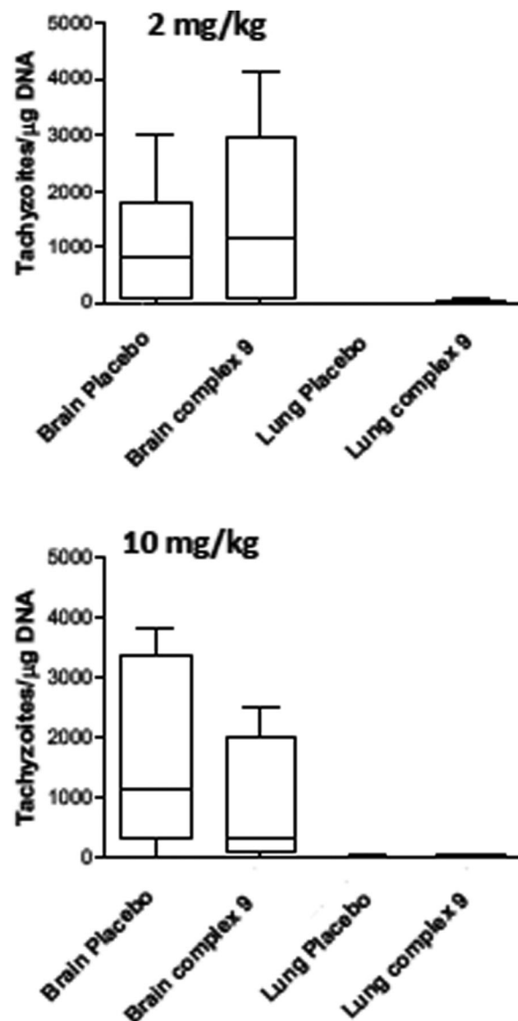
Fig. 6 Box plots of parasite loads (no of tachyzoites/ \mu\text{g DNA} ) in complex 9 treated N. caninum infected Balb/c mice. The drug was applied by oral gavage of either 2 mg kg -1 bodyweight for 5 days (A) or 10 mg kg -1 bodyweight during 5 days. Placebo groups received corn oil only.
