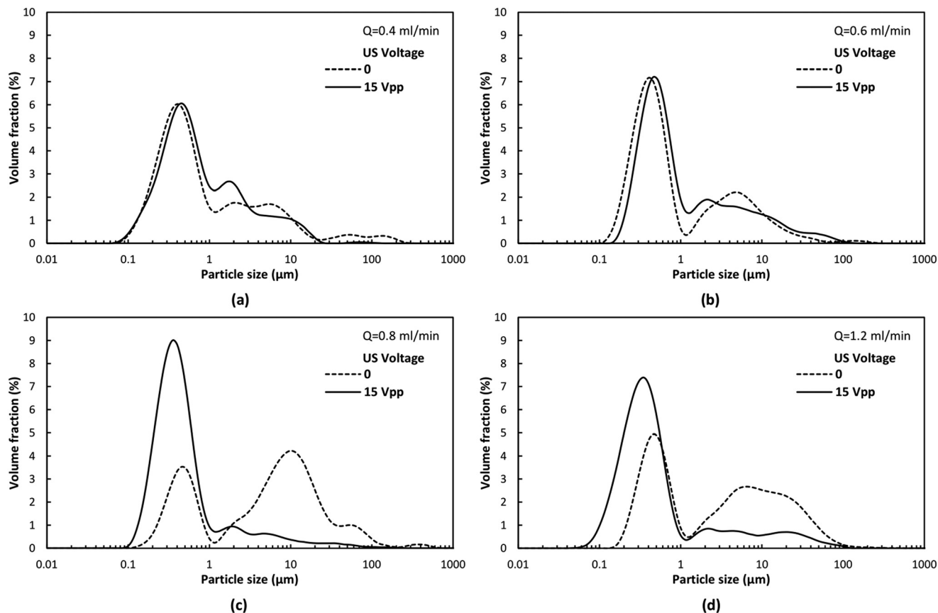
Fig. 8 Effect of US on the \text{CaCO}_3 particle size distribution at different flow rates.
