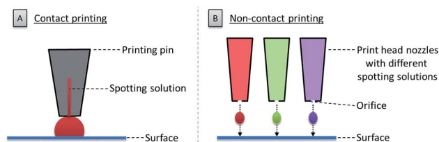
Fig. 3 Schematic illustration of contact (A) and non-contact printing (B).
