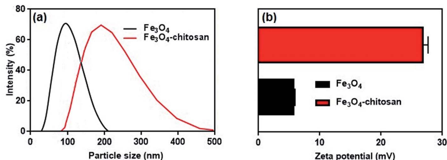
Fig. 8 (a) Hydrodynamic particle size distribution and (b) zeta potential values of \text{Fe}_3\text{O}_4 nanoparticles and \text{Fe}_3\text{O}_4 -chitosan particles.
