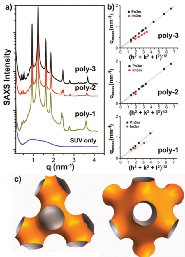
Fig. 21 SAXS data (a,b) for a lipid bilayer containing antimicrobial poly-methacrylates and corresponding real space model (c). Reproduced with permission from ref. 157, copyright 2013, American Chemical Society.
