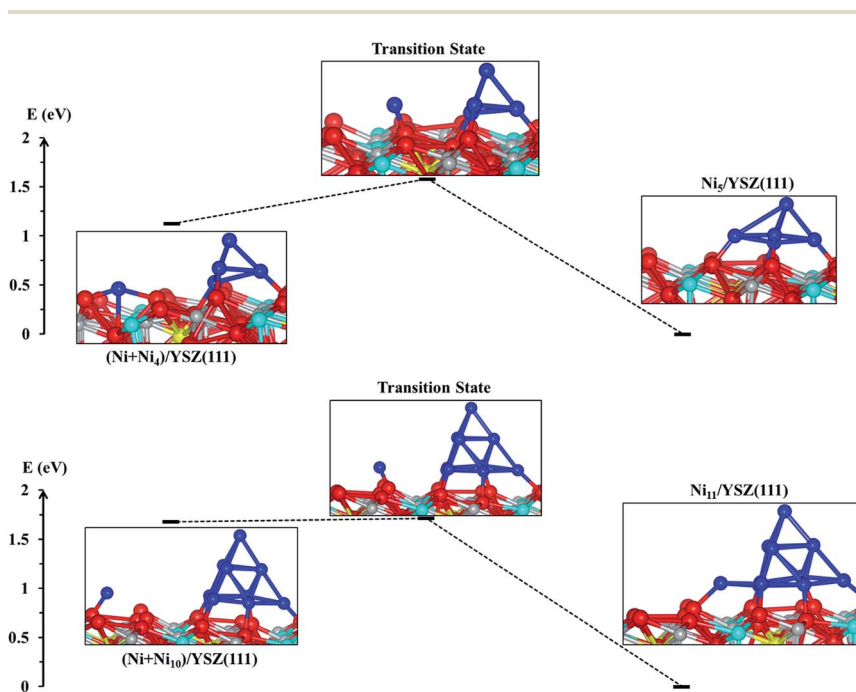
Fig. 7 Energy profile showing two transition states: from state (\text{Ni} + \text{Ni}_4)/\text{YSZ}(111) to \text{Ni}_5/\text{YSZ}(111) and from state (\text{Ni} + \text{Ni}_{10})/\text{YSZ}(111) to \text{Ni}_{11}/\text{YSZ}(111) . Colour key: red, grey, blue and cyan spheres correspond to oxygen, Zr, Ni and Y atoms, respectively. The oxygen vacancy is represented by a yellow sphere.
