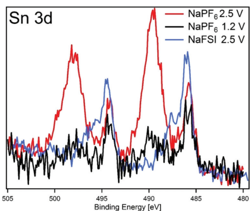
Fig. 7 HAXPES spectra of Sn 3d orbital using photon energy of 2005 eV for: \text{NaPF}_6 charged to 1.2 V (black) and 2.5 V (red) and NaFSI charged to 2.5 V (note NaFSI sample electrolyte contained 5 vol% FEC).
