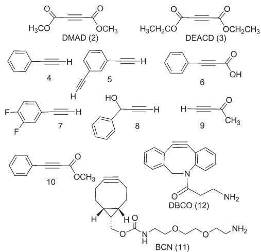
Fig. 1 Commercially available alkyne investigated for their reactivity towards trans,trans,trans -[Pt(N 3 ) 2 (OH) 2 (py) 2 ] (1): DMAD (2), DEACD (3), N -[(1 R ,8 S ,9 s )-bicyclo[6.1.0]non-4-yn-9-ylmethylloxycarbonyl]-1,8-diamino-3,6-dioxaoctane and BCN (11) dibenzocyclooctyne-amine, DBCO (12) were reactive, whereas phenylacetylene (4); 1,3-diethynylbenzene (5); phenylpropionic acid (6); 3,4-difluorophenylacetylene (7) 1-phenyl-2-propyn-1-ol (8); 3-butyn-2-one (9) and 4-phenyl-3-butyn-2-one (10) were not.
