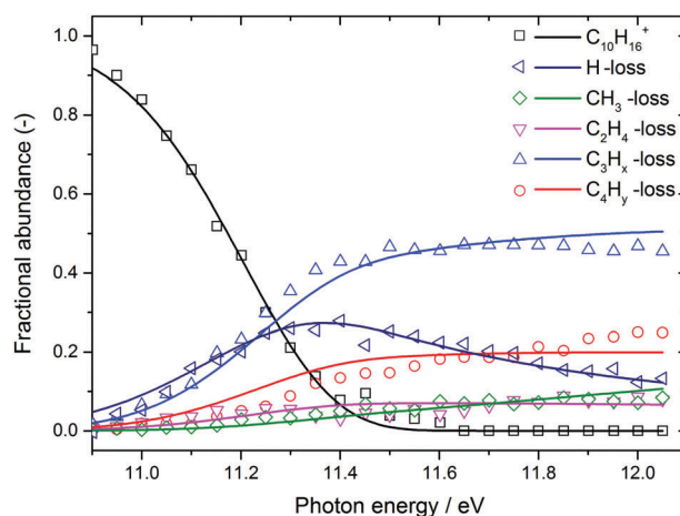
Fig. 4 Adamantane breakdown diagram (open symbols) plotted together with the RRKM model fit (solid lines). Appearance energies derived from the fits are summarised in Table 1.
