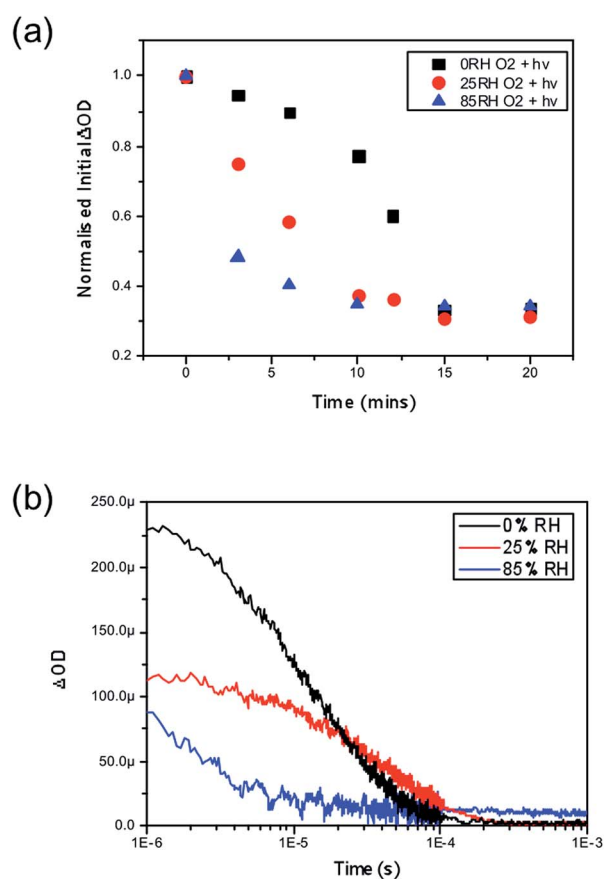
Fig. 4 (a) Normalised transient absorption spectroscopy yield values obtained at 1 μs highlighting the degradation rate differences between CH 3 NH 3 PbI 3 pre-treated under no moisture, 25% RH and 85% RH upon exposure to both oxygen and light at t = 0 . (b) Kinetic decays obtained after five minutes of exposure to oxygen and light for all three samples. All films were excited with a pump wavelength of 567 nm and an average power of 23 μJ cm -2 and a probe wavelength of 1600 nm was employed to probe the resulting holes in spiro-OMeTAD.
