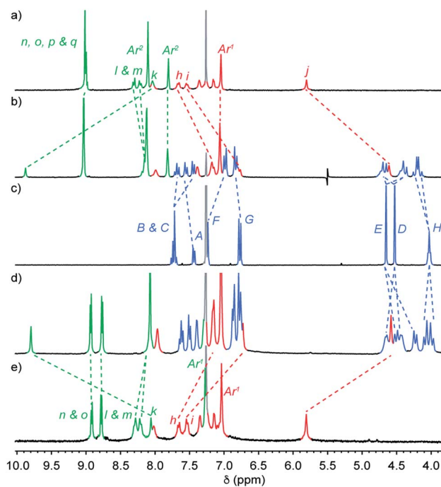
Fig. 1 Partial ^1H NMR ( CDCl_3 , 300 MHz, 298 K) of (a) dyad axle 4 , (b) [2]rotaxane 4C3 , (c) macrocycle 3 , (d) [3]rotaxane 5C3_2 and (e) triad axle 5 . Peak assignments as shown in Scheme 1. Residual solvent signals are indicated in light grey.
