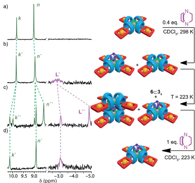
Fig. 3 Partial 1 H NMR (CDCl 3 , 300 MHz) of (a) pentad [5]rotaxane 6C 34 (298 K); (b) 6C 34 + DABCO (0.4 equiv., 298 K); (c) 6C 34 + DABCO (0.4 equiv., 223 K); (d) 6C 34 + DABCO (1 equiv., 223 K). Peak assignments as shown in Scheme 1. Primed (') and doubly primed labels refer to signals attributed to [(6C 34 )L] and [(6C 34 ) 2 L] respectively. Cartoon representations have been included to aid clarity but are not intended to be representative of the structures of the complexes formed. 28
