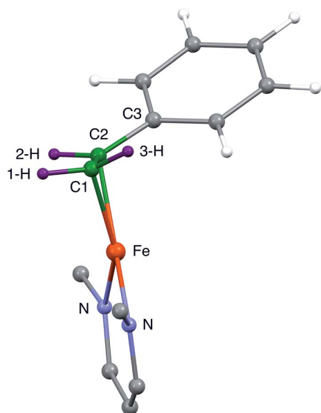
Fig. 3 Side view of the core of the DFT model of 1, showing that the phenyl group is displaced away from the dicitiminate supporting ligand. This tilts the plane of the alkene and also places C2 further than C1 from Fe.
