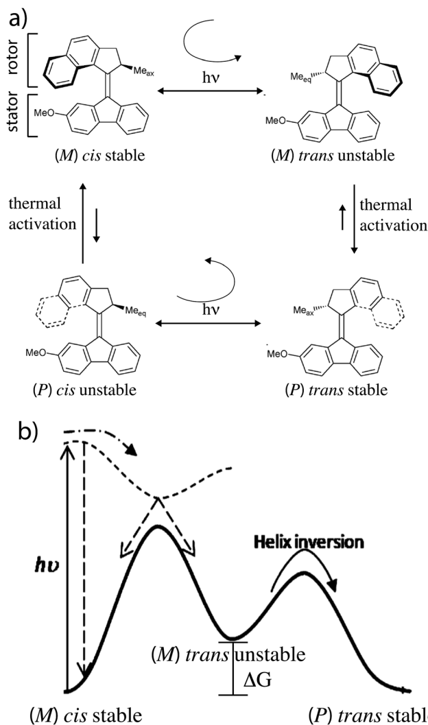
Fig. 1 (a) Light driven molecular motor cycle designed by Ben Feringa and colleagues. The design is based on over-crowded alkenes, where the notation (M) or (P) denotes left (Minus) or right (Positive) helicity. For convenience we designate the bottom part of the molecule as the “stator” and the top part as the “rotor”. The subscript on the methyl group (Me) at the chiral carbon atom of the rotor denotes whether the orientation of the methyl is axial (ax) or equatorial (eq). (b) Ground (solid curve) and excited state (dashed curve) energy surfaces for motion of the rotor relative to the stator of the motor in (a).
