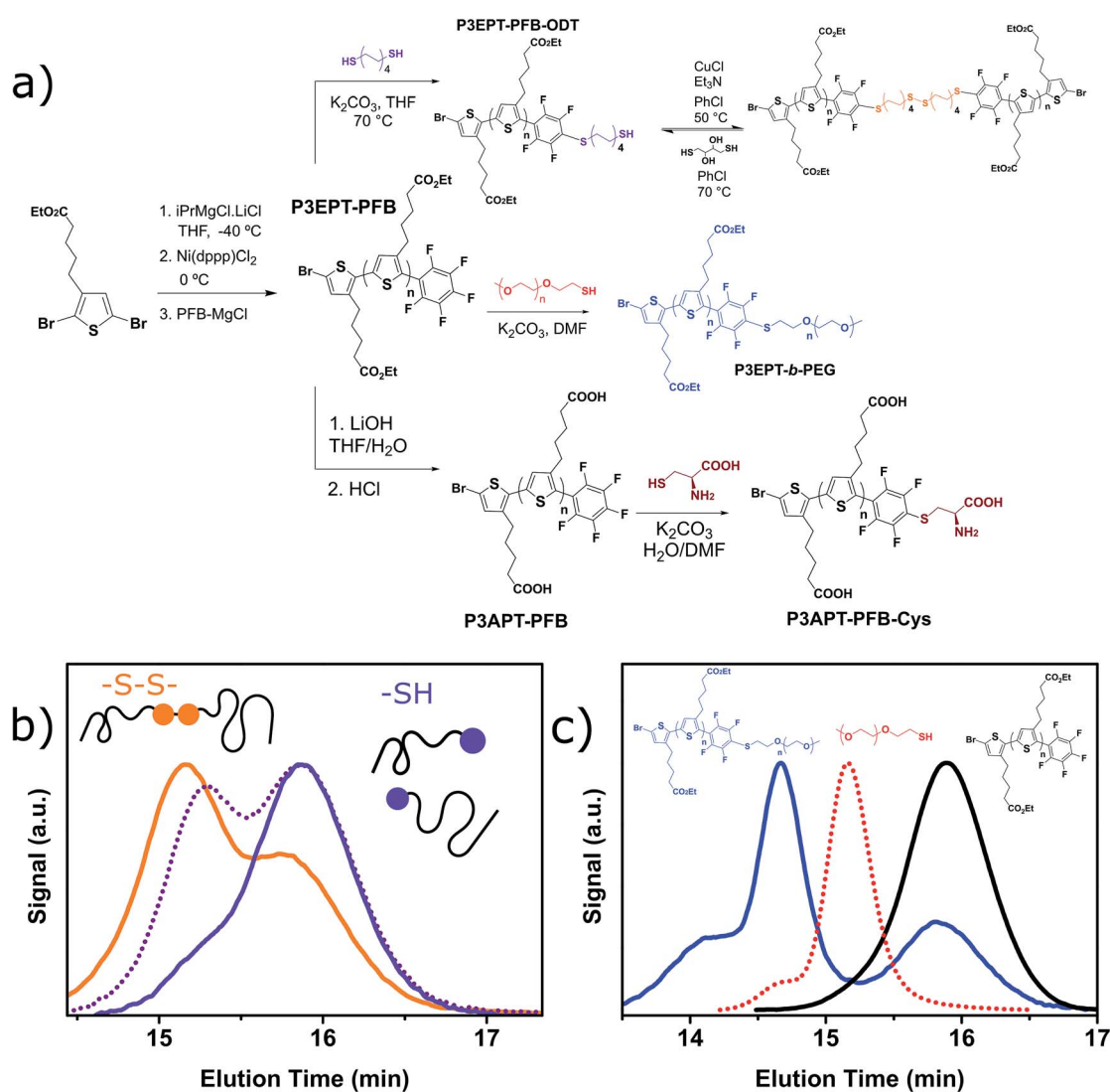
Fig. 5 (a) Synthesis of P3EPT-PFB and P3APT-PFB with model “click” reactions performed post-polymerization. (b) Gel permeation chromatography elugram ( 80 °C in chlorobenzene) of P3EPT-PFB-ODT in the thiol (purple) and disulfide (orange) forms. The dotted purple line illustrates partial reduction of the disulfide link (c) gel permeation chromatography elugram ( 80 °C in chlorobenzene) of P3EPT-PFB (black), mPEG-SH (red), and P3EPT- b -PEG (blue). Traces for all elugrams are obtained from a 450 nm diode array detector, except mPEG-SH which was measured using a refractive index detector.
