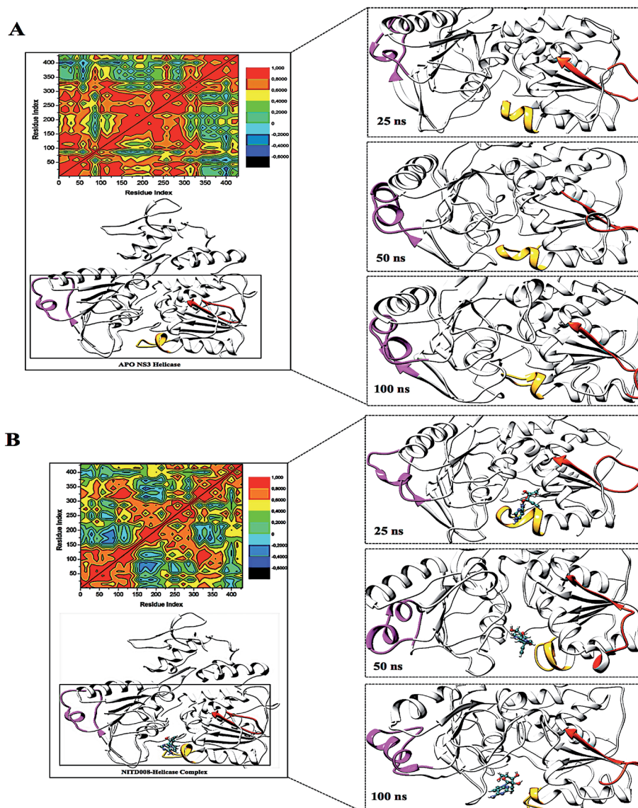
Fig. 7 Structural flexibility of the P-loop (196–203), RNA-binding loop (244–255), and the _{310} helix (339–348) along the trajectory. The RNA-binding loop (orange) showed the loop shifting down in the APO structure but an upward shift in the NITD008-helicase complex. The P-loop (yellow) shifted away from the active site in the bound complex but closed in on the active site when no ligand was present. In the APO structure, the helix-loop-helix stayed, with vibrational movement during the simulation, although, in the bound complex, the _{310} helix (pink) was modified into a \alpha -helix due to ligand motional shifts further into the hydrophobic pocket.
