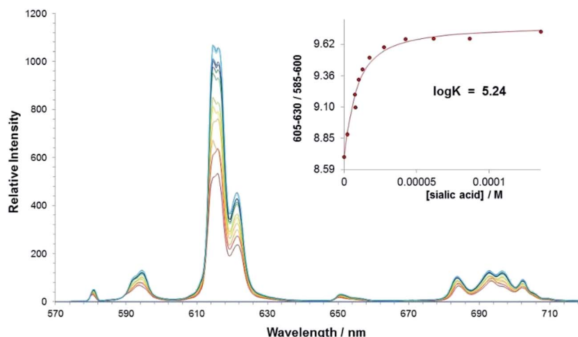
Fig. 5 Variation of the europium(III) emission profile of [Eu·L 1 ] + as a function of added sialic acid. (5 \mu\text{M} , \lambda_{\text{exc}} = 352 \text{ nm} , MeOH). Inset shows fit to experimental data, following iterative least squares fitting to a 1 : 1 binding model.
