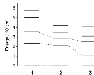
Fig. 4 Energy level diagram of the splitting of the ground {}^4F term for a free \text{Co(II)} ion in the ligand field of 1 , 2 and 3 . This diagram was extracted from ab initio spin-free calculations, and each black line corresponds to a spin-free quartet without SOC. The orbital degeneracy is broken down by the actual geometry, resulting in seven quartets for each complex.
