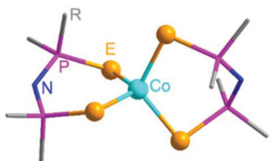
Fig. 1 Molecular structure diagram of Co([EPR 2 ) 2 N] 2 ( E = \text{S, Se, Te} ; R = \text{Ph, } ^i\text{Pr} ). The hydrogen atoms and the R groups are not shown for clarity.
