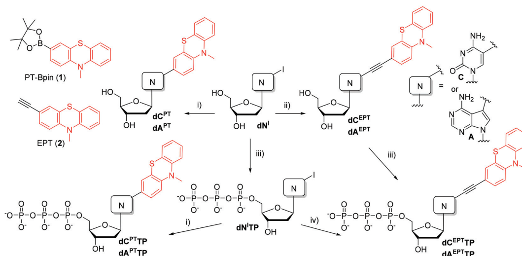
Scheme 1 Reagents and conditions: (i) PT-Bpin ( 1 ), Pd(OAc) 2 , TPPTS, Cs 2 CO 3 , AN/H 2 O (1:1), 50 °C, 40 min; (ii) EPT ( 2 ), Pd(PPh 3 ) 2 Cl 2 , CuI, Et 3 N, DMF, 75 °C, 1 h; (iii) 1. POCl 3 , PO(OMe) 3 , 0 °C, 3 h; 2. (NH 4 Bu 3 ) 2 H 2 P 2 O 7 , Bu 3 N, DMF, 0 °C, 1.5 h; 3. TEAB; (iv) EPT ( 2 ), Pd(OAc) 2 , CuI, TPPTS, Et 3 N, AN/H 2 O (1:1), 75 °C, 1 h.
