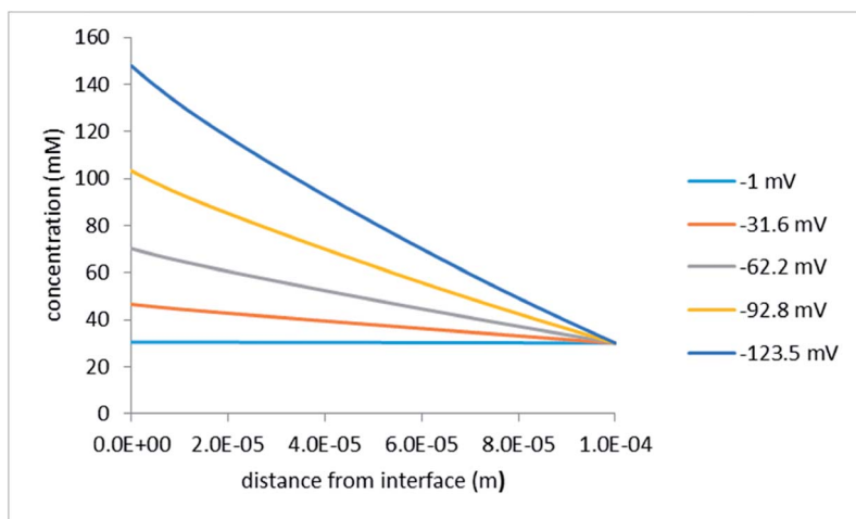
Fig. 9 Concentration distribution along the z -axis at the upper right cell corner (see Fig. 2); the legend indicates the applied voltages; the half-distance between the hole centers is 15\text{ }\mu\text{m} .
