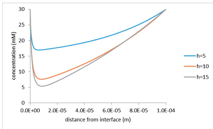
Fig. 8 Concentration distribution along the z -axis at the hole edge; \phi_0 = 200 mV; the legend indicates half-distance between the hole centers in micrometers.
