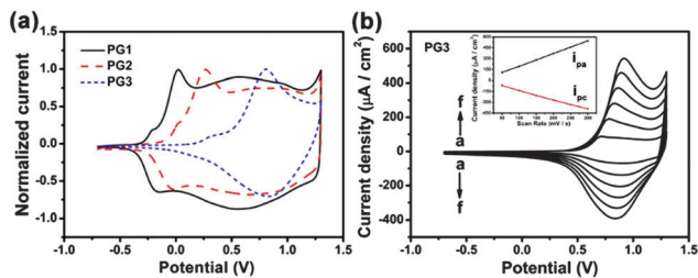
Fig. 2 (a) Single scan cyclic voltammograms of different films at 100 mV s -1 in 0.1 M TBAPF 6 /ACN: PG1 (black, solid line), PG2 (red, dashed line), and PG3 (blue, short dashed line). (b) Scan rate dependence of the PG3 film in 0.1 M TBAPF 6 /ACN at (a) 50, (b) 100, (c) 150, (d) 200, (e) 250 and (f) 300 mV s -1 (inset is the plot of scan rate with anodic (i pa ) and cathodic (i pc ) peak currents).
