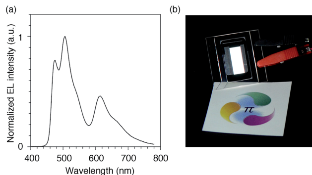
Fig. 9 White OLED with a single-layer architecture. (a) An electroluminescence spectrum at a current density of 0.1 \text{ mA cm}^{-2} . (b) A picture of the device with an emitting area of 16.6 \text{ mm} \times 6 \text{ mm} . The sheet under the device is showing a color reference printed on white paper, and the original colors can be found at http://www.jst.go.jp/erato/isobe/ .
