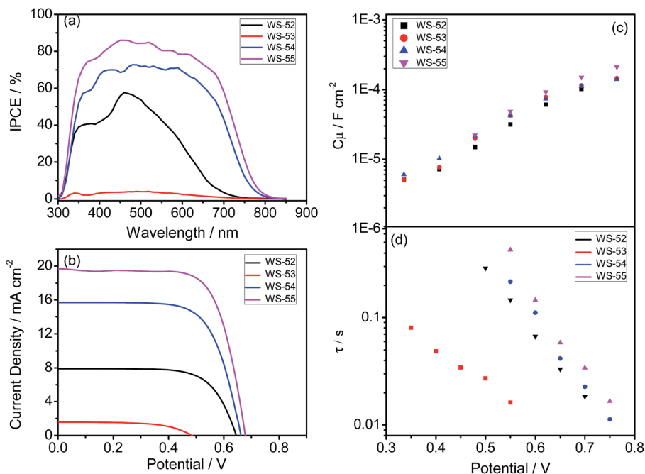
Fig. 3 IPCE (a) and J - V curves (b), and bias potential against TiO 2 capacitance (c) and electron lifetime (d) in DSSCs sensitized by WS-52, WS-53, WS-54 and WS-55.
