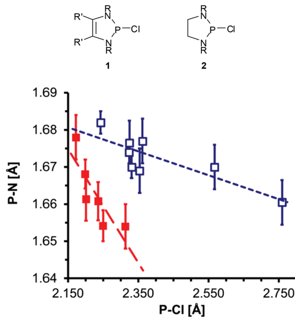
Fig. 1 Plot of P–Cl distances vs. average PN distances in selected P-chloro-1,3,2-diazaphospholenes 1 (open squares; R = alkyl, aryl, R' = H, Me) and 1,3,2-diazaphospholidines 2 (filled squares; R = alkyl, aryl). Error bars denote ranges of ±3σ; dashed lines represent the results of linear regression analyses.
