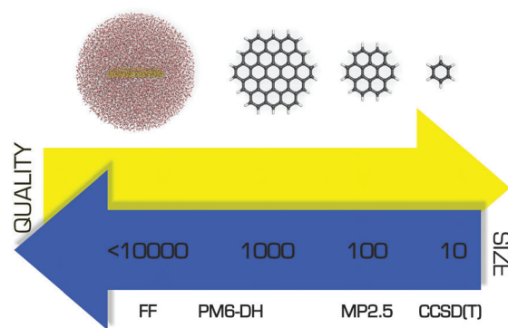
Fig. 5 Comparison of several theoretical approaches with respect to the size of the system that can be treated efficiently and the quality of the resulting description.
