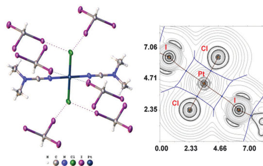
Fig. 1 Left: View of fragment 1a · (\text{CHI}_3)_6 from \mathbf{1a}\cdot\frac{1}{2}\text{CHI}_3\cdot\frac{1}{2}\text{CHI}_3 . Thermal ellipsoids are shown with 50% probability and short contacts are indicated by dotted lines. Coordinates of this fragment were applied in further DFT calculations. Right: Contour line diagram of the Laplacian distribution \nabla^2\rho(r) (cross-section along the plane \text{Pt-Cl-I} ) was received as a result of the topological analysis of the electron density distribution in the model structure. Bond paths are shown as brown lines, selected zero-flux surfaces – as blue lines, bond critical points (3, -1) are shown in blue, nuclear critical points (3, -3) – in pale brown, length unit – Å.
