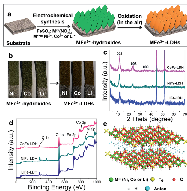
Fig. 1 (a) Scheme of the synthetic route to the MFe-LDH (M = Ni, Co and Li) nanoarrays; (b) photograph of the MFe-LDH nanoarrays growing on the Ni foam before and after self-oxidation in the air; (c) XRD patterns and (d) XPS spectra of the MFe-LDH (M = Ni, Co and Li) nanoplatelet arrays; (e) structure model of MFe-LDH.
