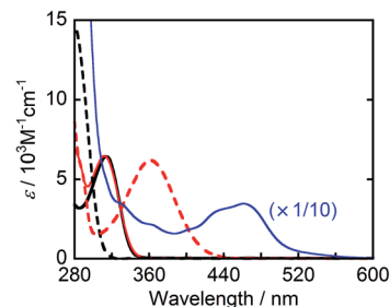
Fig. 1 UV-vis absorption spectra of \text{BIH} (black solid line), \text{BI}^{+} (black broken line), \text{BI(OH)H} (red solid line), \text{BI(O}^{\ominus})^{+} (red broken line), and \text{Ru}_2\text{-Ru(CO)} (blue line, 1/10 intensity) in DMF-TEOA (4 : 1 v/v).
