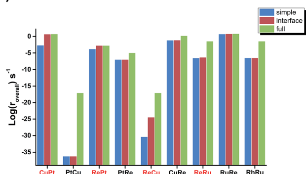
Fig. 3 Activity ( \log(r_{\text{overall}}) ) comparisons of nine bi-phase surfaces among (a) those from the upper phase, lower phase and bi-phase surfaces, respectively, (b) the simple, interface and full kinetic models, where the reactive-noble bi-phase surfaces are highlighted in red.
