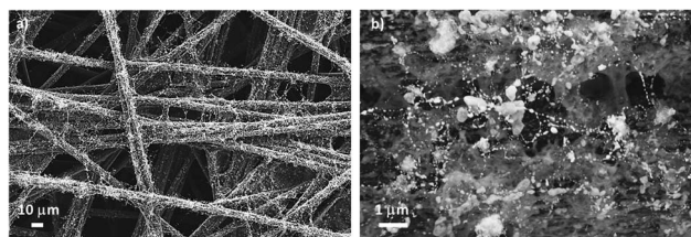
Fig. 5 SEM images of electrospayed 46 wt% Pt-CNT–C 6 H 10 O 5 composites, showing direct contact between the electrolyte particles with the carbon nanotubes: (a) low and (b) high magnification.
