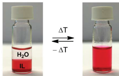
Fig. 8 Reversible formation of a homogeneous phase when increasing the temperature above the cloud point ( 55\text{ }^\circ\text{C} for a pure water/ionic liquid system in a 1:1 ratio). 44 A coloring agent (methyl red sodium salt) was dissolved in the transparent ionic liquid phase to help the visualization. The density of the [Hbet][Tf_2N] liquid is higher than that of water.
