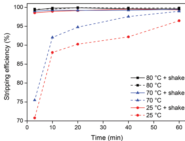
Fig. 9 Stripping kinetics and the influence of shaking (1500 rpm) are shown for 25\text{ }^\circ\text{C} , 70\text{ }^\circ\text{C} and 80\text{ }^\circ\text{C} with 1\text{ M} HCl. The cloud point temperature is 74\text{ }^\circ\text{C} and so at 80\text{ }^\circ\text{C} the system is one homogeneous phase which explains the efficient stripping without shaking. For 25\text{ }^\circ\text{C} and 70\text{ }^\circ\text{C} it consists of two phases, a water phase and an ionic liquid phase, making shaking essential for an efficient stripping process.
