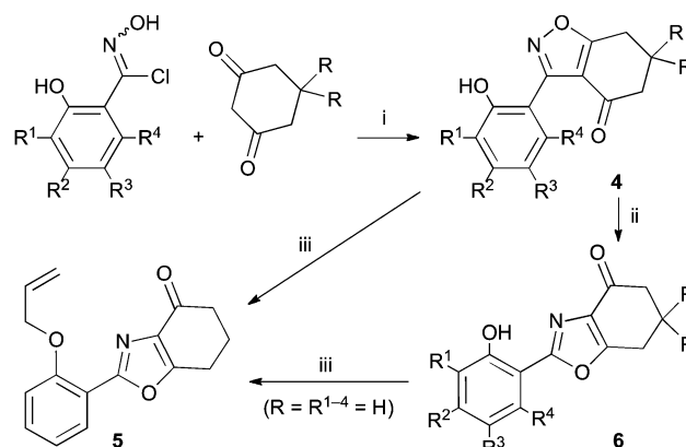
Scheme 2 Synthesis and rearrangement of 3-aryltetrahydrobenzisoxazoles 4 . Reagents: (i), NaOi-Pr, i -PrOH; (ii), Cs 2 CO 3 , THF reflux; (iii), H 2 C=CHCH 2 Br, Cs 2 CO 3 , THF reflux.
