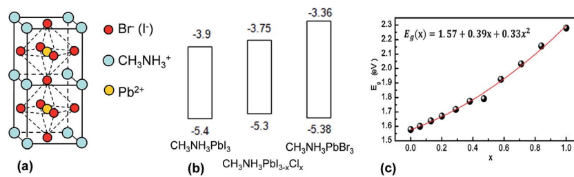
Fig. 14 Structure and energy levels for perovskites used in solar cells. (a) Unit cell for CH 3 NH 3 PbI 3 and CH 3 NH 3 PbBr 3 perovskites. (b) Energy levels for CH 3 NH 3 PbI 3 , CH 3 NH 3 PbI 3-x Cl x and CH 3 NH 3 PbBr 3 . The energy levels for the latter were taken from ref. 209, 210 and 211 respectively. (c) Variation of E_g with Br composition for CH 3 NH 3 Pb(I 3-x Br x ) 3 . (c) reproduced with permission from ref. 208.
