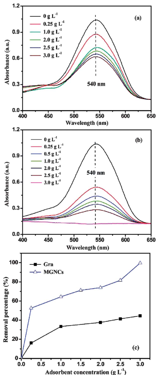
Fig. 10 UV-Vis absorption of the solutions after treated with (a) different loadings of graphene (Gra), (b) different loadings of MGNCs, and (c) \text{Cr(VI)} removal percentage based on different loadings of Gra and MGNCs. ( [\text{Cr(VI)}] = 1000 \mu\text{g L}^{-1} , pH 7, treatment time: 5 min). Reproduced with permission from ref. 242, copyright (2011) American Chemical Society.
