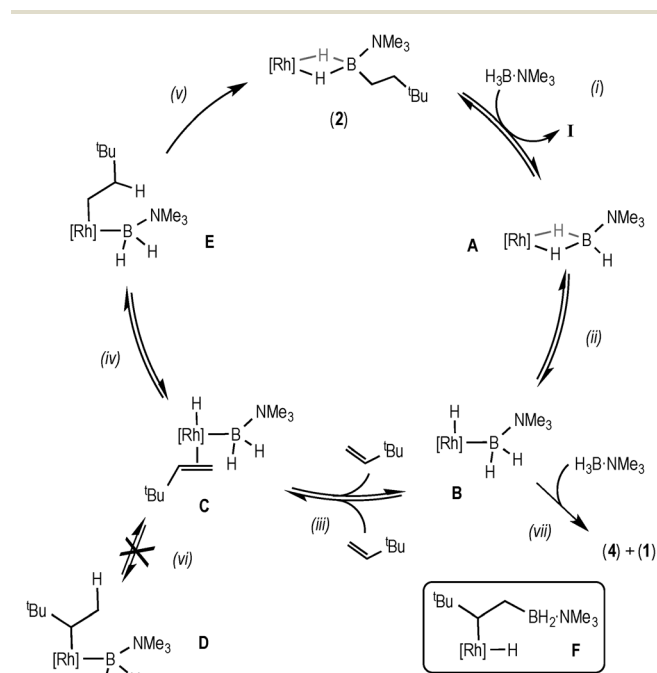
Scheme 6 Proposed mechanism for the catalytic hydroboration using data from the early phase of catalysis. [Rh] = [\text{Rh}(\text{xantphos})]^+ .
